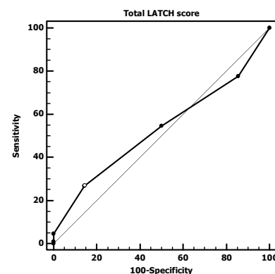
Figure 1: ROC curve
